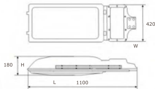
Lamp Size: (Unit: mm)
