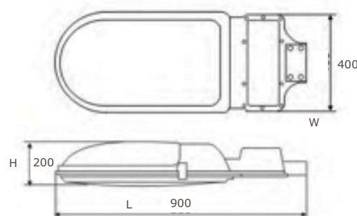
Lamp Size: (Unit: mm)
