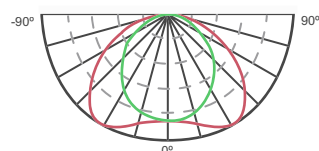
Light distribution curve:
