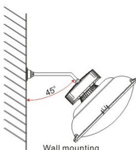
Wall mounting
