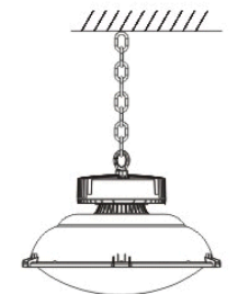
Hanging chain installation
