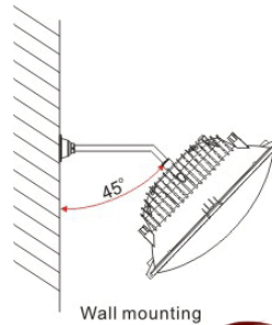
Wall mounting
