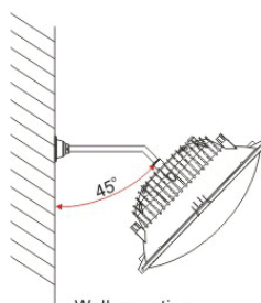
Wall mounting
