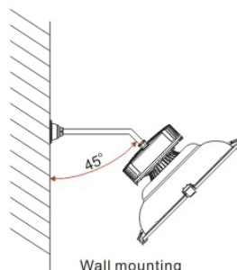
Wall mounting
