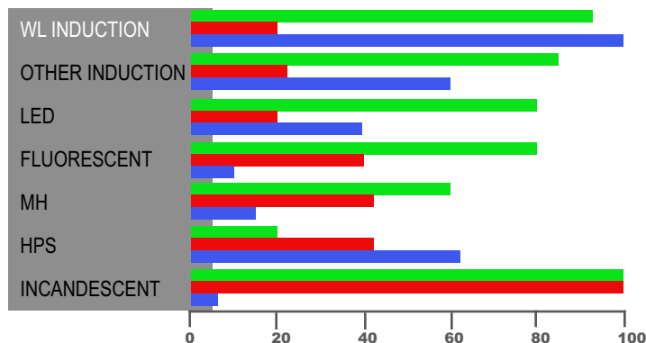
INDUCTION CFL MH HPS GLARE / FLICKER COMPARISON
