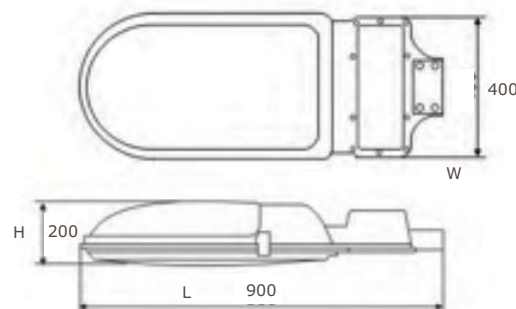
Lamp Size: (Unit: mm)
