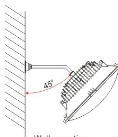
Wall mounting
