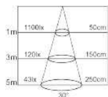
Lux diagram
