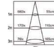
Lux diagram
