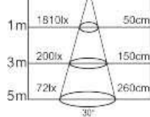
Lux diagram
