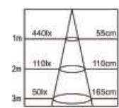
Lux diagram
