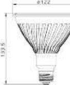
Dimension
